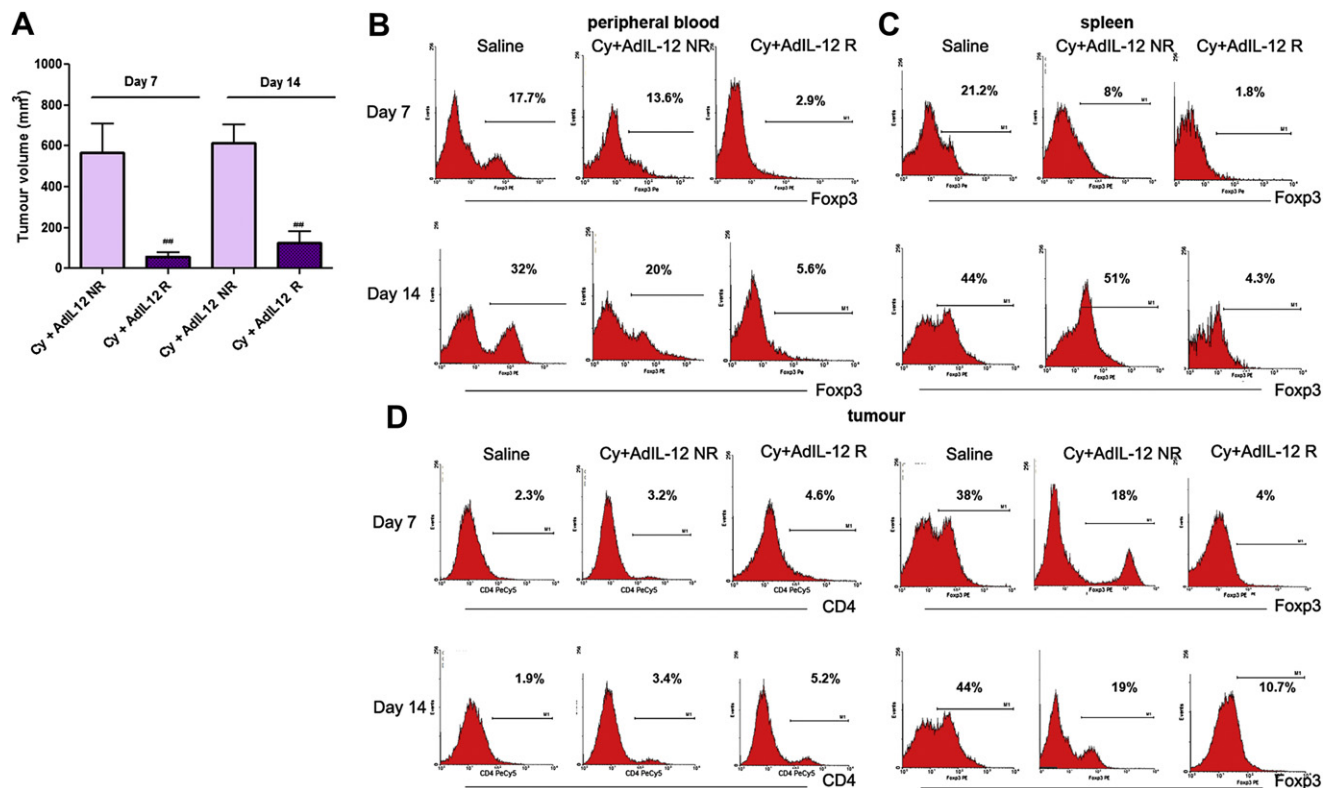
Fig. 1 – Assessment of Tregs in mice R (responder) and NR (non-responders) to combined treatment Cy + AdIL-12 in s.c. CT26 tumour model. (A) Tumour volume in R and NR mice. BALB/c mice ( n = 35 ) were s.c. inoculated with 5 \times 10^5 CT26 cells into the right flank (day 0) and tumours were allowed to reach 85 mm 3 before the treatment began. Animals were treated with Cy (50 mg/kg i.p., day 8) + AdIL-12 ( 10^9 TCID50 i.t., day 9) ( n = 12 ) or with saline ( n = 6 ). Tumour growth was assessed twice a week by calliper. Tumour volumes at days 7 and 14 after treatment are expressed as mean (bars, SEM). The experiment was performed four times. Mann-Whitney test, Cy + AdIL-12 NR vs. Cy + AdIL-12 R: ( \#\#p < 0.01 ). Percentage of CD4 + CD25 + Foxp3 + /CD4 + cells in peripheral blood (B) or spleen (C) of R and NR mice. Mann-Whitney test, Peripheral blood, day 7 and day 14: Cy + AdIL-12 R vs. saline ( ^{**}p < 0.01 ) and vs. Cy + AdIL-12 NR ( \#p < 0.05 ); Cy + AdIL-12 NR vs. saline ( *p < 0.05 ); day 14: Cy + AdIL-12 R vs. saline ( ^*p < 0.05 ) and Cy + AdIL-12 NR ( ^*p < 0.05 ). (D) Percentage of tumour-infiltrating CD4 + T cells (left) and CD4 + CD25 + Foxp3 + /CD4 + cells (right). Mann-Whitney test, CD4 + T cells, day 7: Cy + AdIL-12 R vs. saline, ( ^*p < 0.05 ); day 14: Cy + AdIL-12 R vs. saline and Cy + AdIL-12 NR ( \#p < 0.05 ); Cy + AdIL-12 NR vs. saline ( ^*p < 0.05 ). CD4 + CD25 + Foxp3 + /CD4 + cells, day 7: Cy + AdIL-12 R vs. saline, ( ^*p < 0.05 ); day 14: Cy + AdIL-12 R vs. saline and Cy + AdIL-12 NR ( \#p < 0.05 ). The results shown represent four independent experiments.
